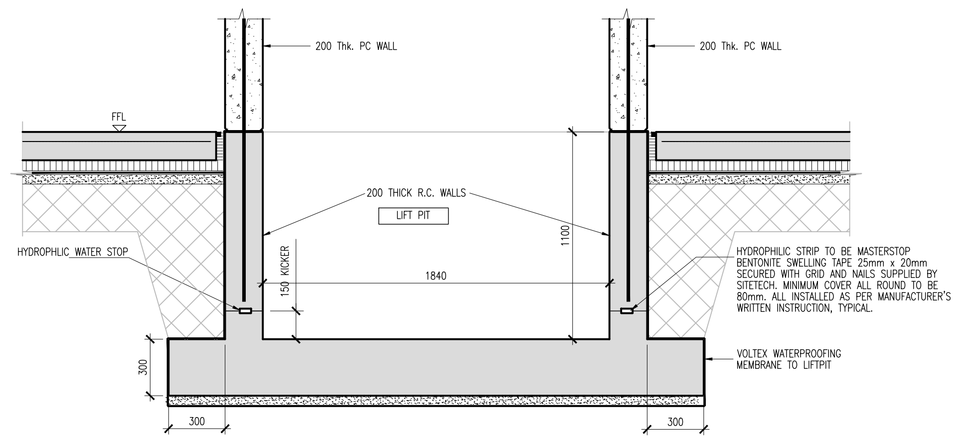
TYPICAL APARTMENT FOUNDATION SECTION 3 (1:20)
