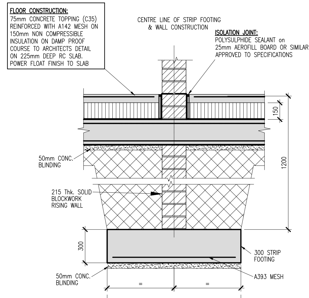
TYPICAL APARTMENT FOUNDATION SECTION 6 (1:20)
