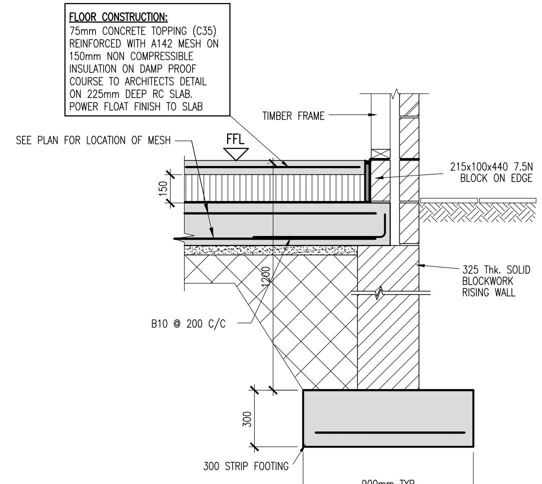
TYPICAL APARTMENT FOUNDATION SECTION 7 (1:20)
