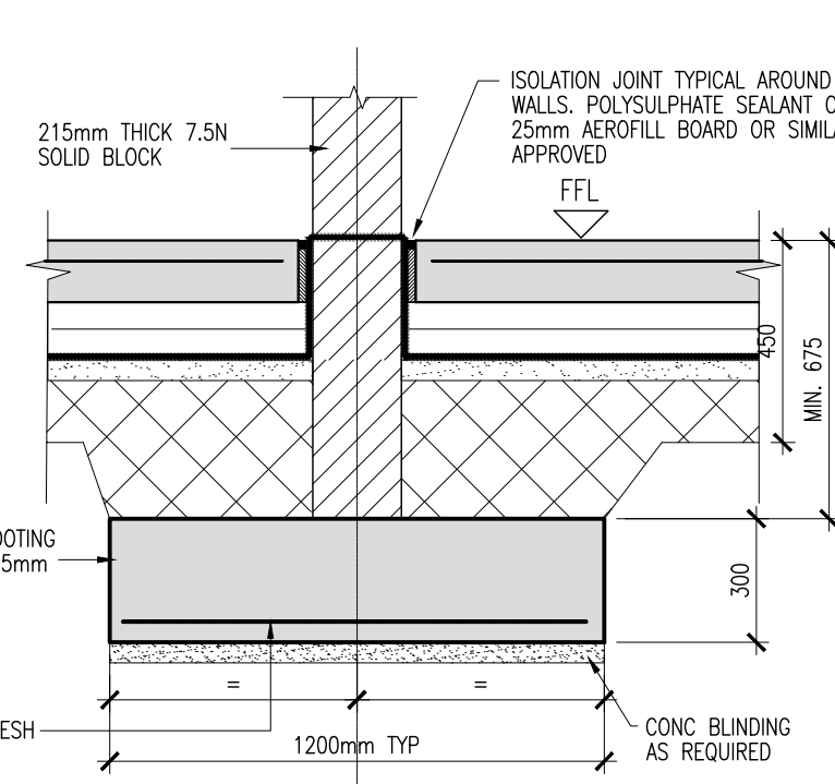
TYPICAL HOUSE FOUNDATION DETAIL 2 (1:20)
