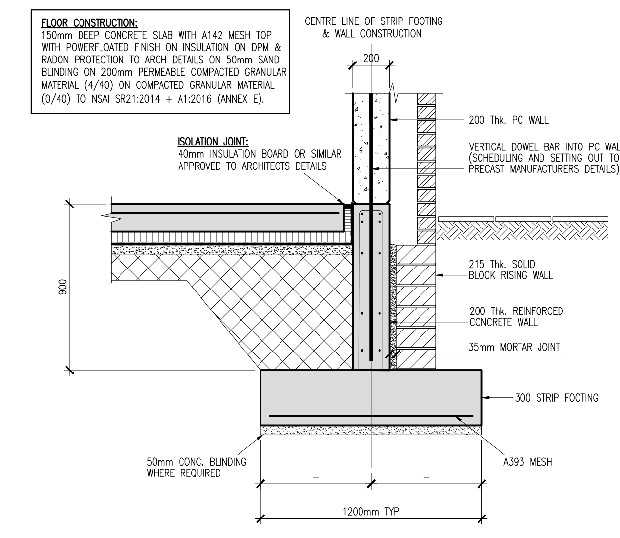
TYPICAL APARTMENT FOUNDATION SECTION 5 (1:20)
