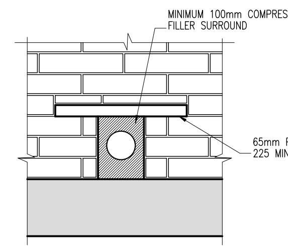
SERVICES ABOVE FOUNDATIONS (1:20)
