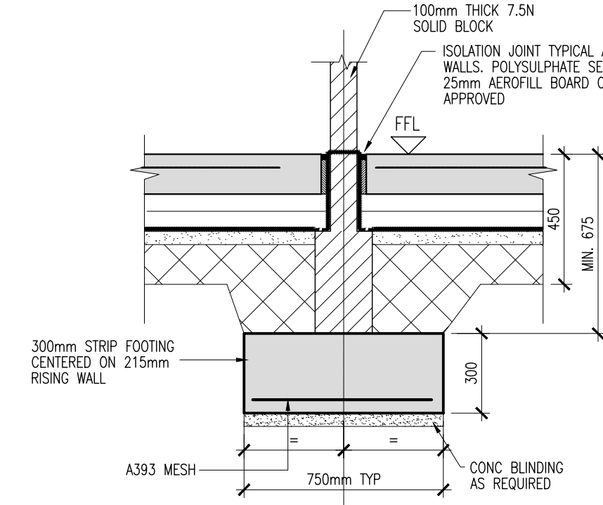
TYPICAL HOUSE FOUNDATION DETAIL 3 (1:20)
