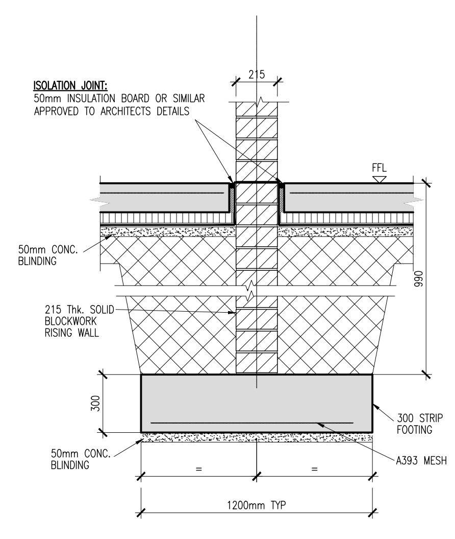
TYPICAL APARTMENT FOUNDATION SECTION 2 (1:20)
