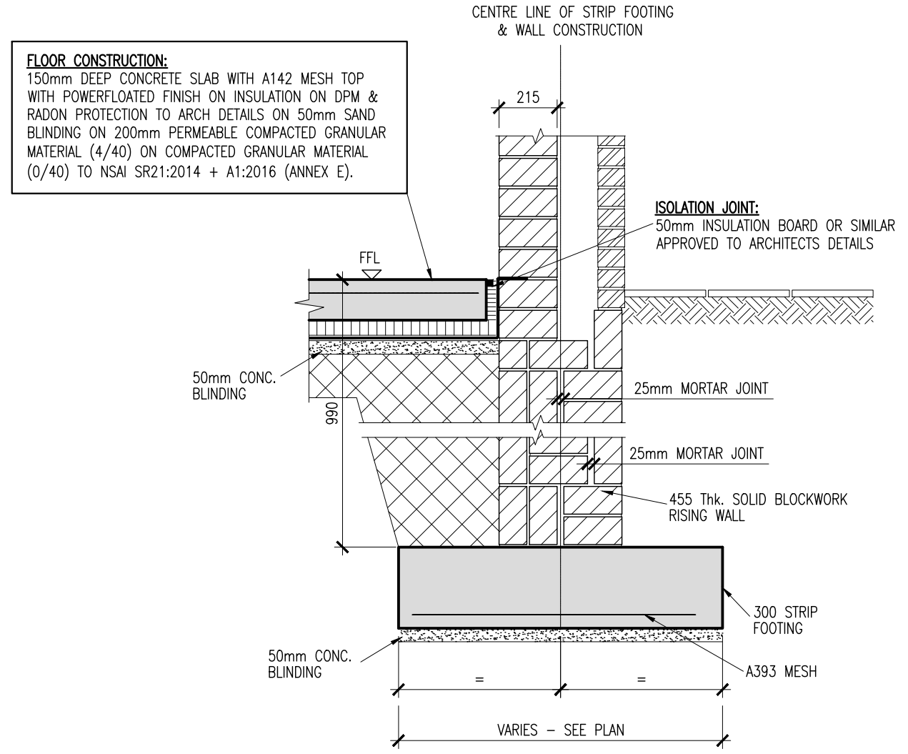
TYPICAL APARTMENT FOUNDATION SECTION 1 (1:20)
